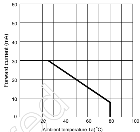
Fig.2 Forward current derating curve vs. ambient temperature
