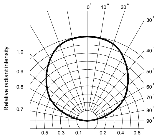
Fig.6 Radiation diagram
